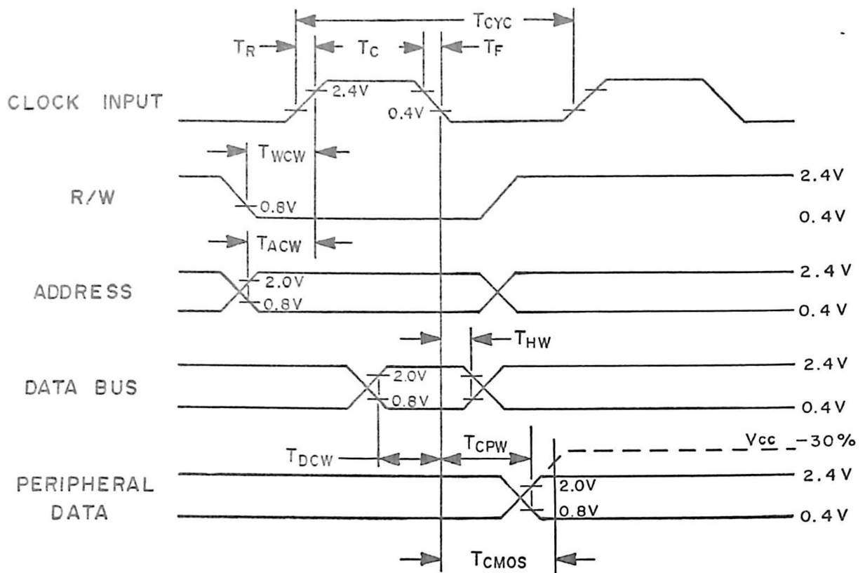
WRITE TIMING CHARACTERISTICS
